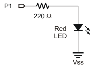
LED Indicator for Right IR Pair
